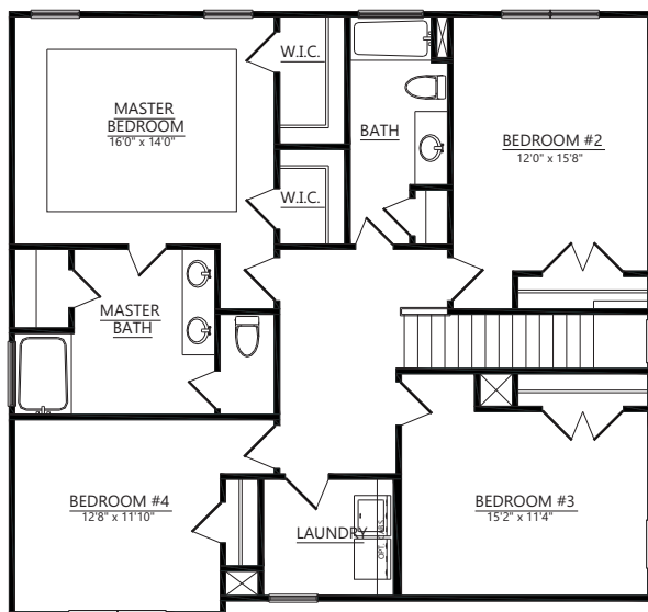
SECOND FLOOR LAYOUT
