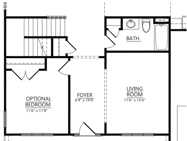
OPT. BEDROOM W/ FULL BATH
