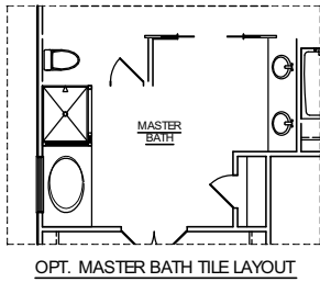
OPT. MASTER BATH TILE LAYOUT
