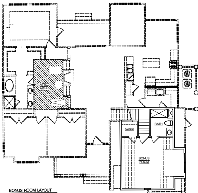
BONUS ROOM LAYOUT
